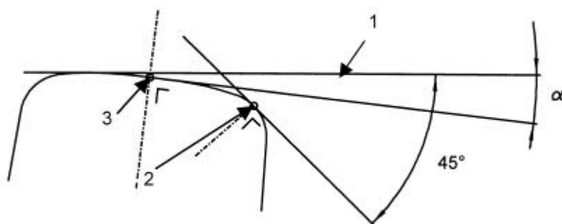
(b) Detailed section of railhead, showing reference point A and B' ( \alpha :angle of rail inclination)
